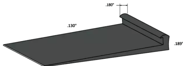
MET-02 LVT to Carpet Transition
