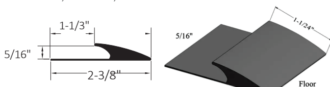
EG-XX-G 5/16" material to floor
