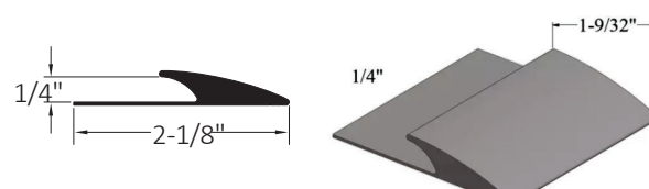
EG-XX-H 1/4" material to floor
