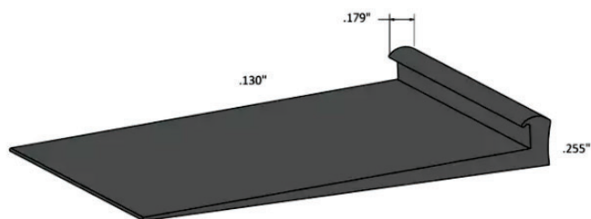
ME-001 LVT to Carpet Transition
